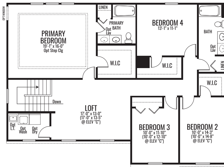
STANDARD SECOND FLOOR
