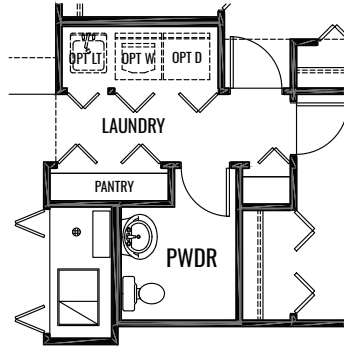
OPTIONAL LAUNDRY TUB (at slab)
