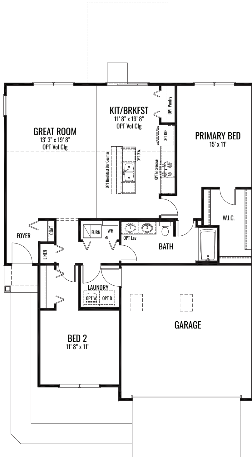
FIRST FLOOR
