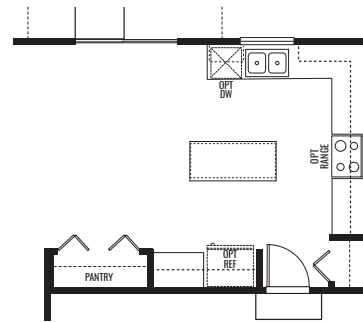
OPT. ISLAND 5' W/ EXTENDED COUNTERTOP
