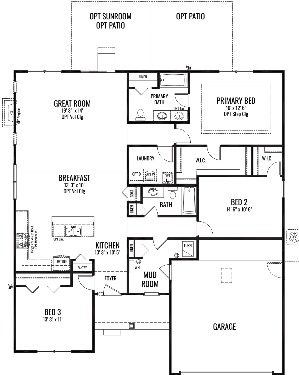
FIRST FLOOR
