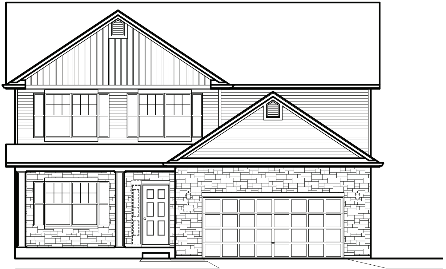
ELEVATION "D"
